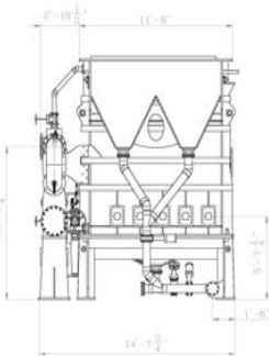
RIGHT VIEW
