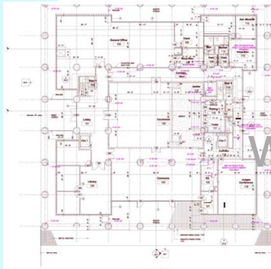
FIRST FLOOR PLAN - PLUMBING
